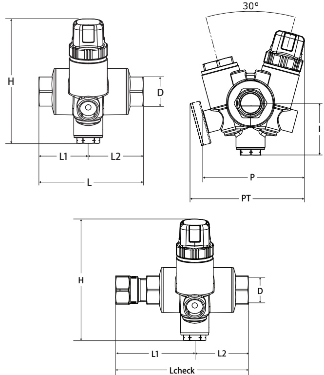
TB-120G with Optional Check Valve
