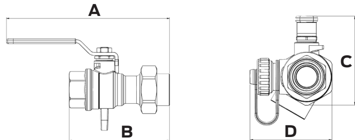
Hot Valve
