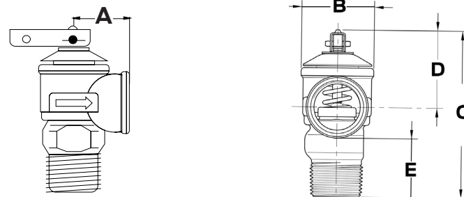
Relief Valve
