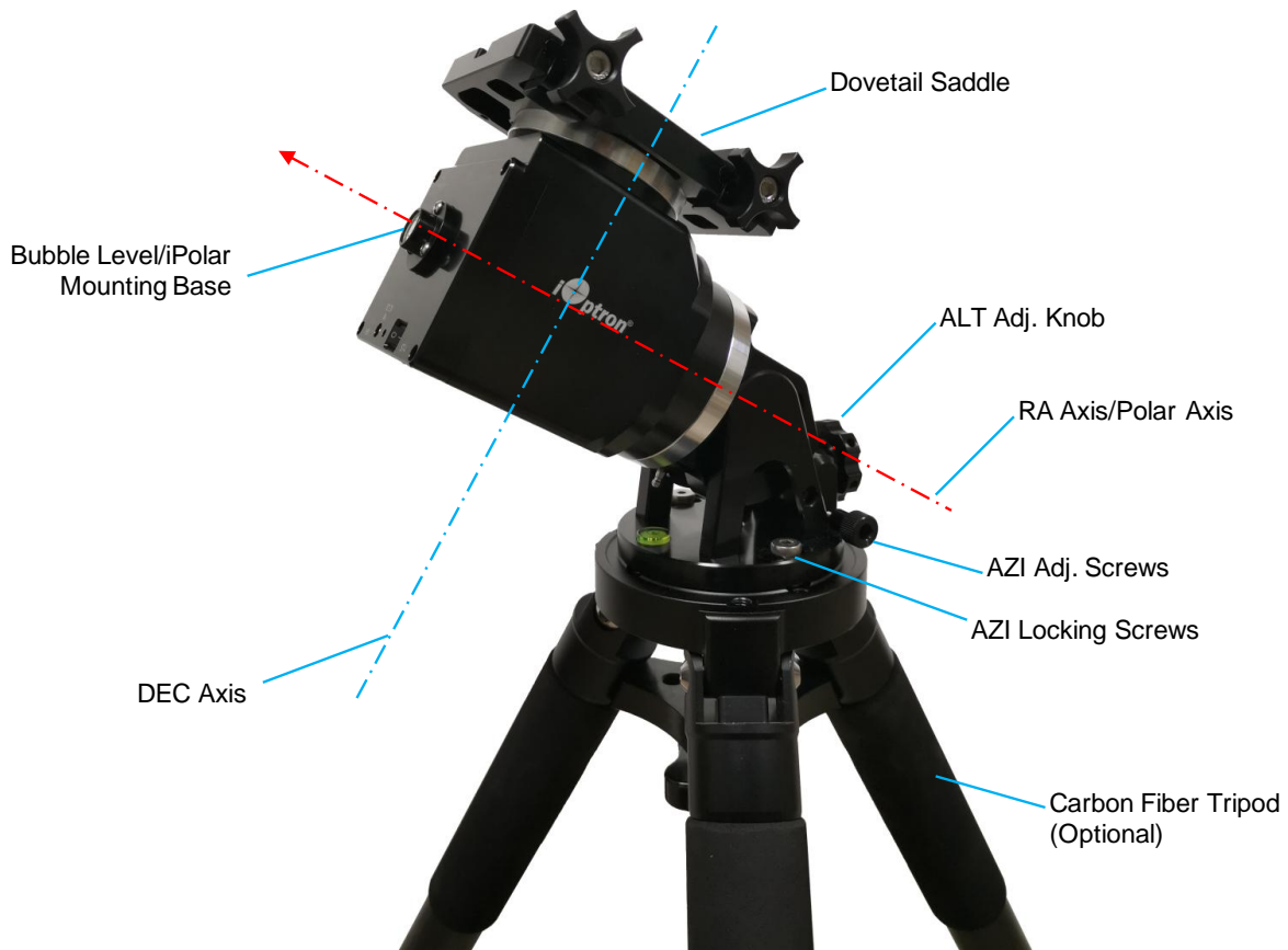
Figure 1. HAE mount assembly
