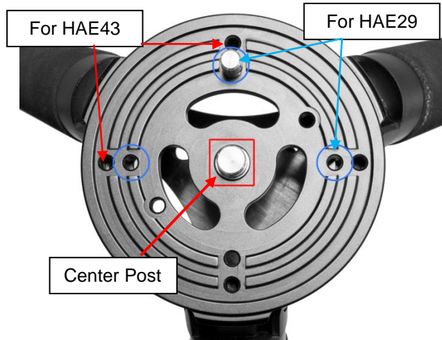
Figure 9. Carbon fiber tripod
