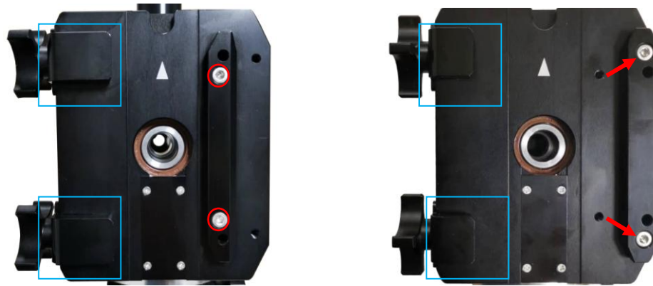
Figure 15. Change dovetail saddle from Vixen (right) to Loasmandy-D (right)
