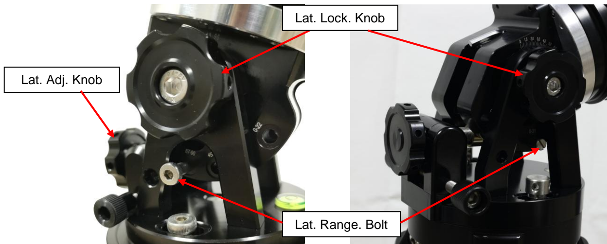
Figure 12. HAE latitude range settings for HAE29 (left) and HAE43 (right)
